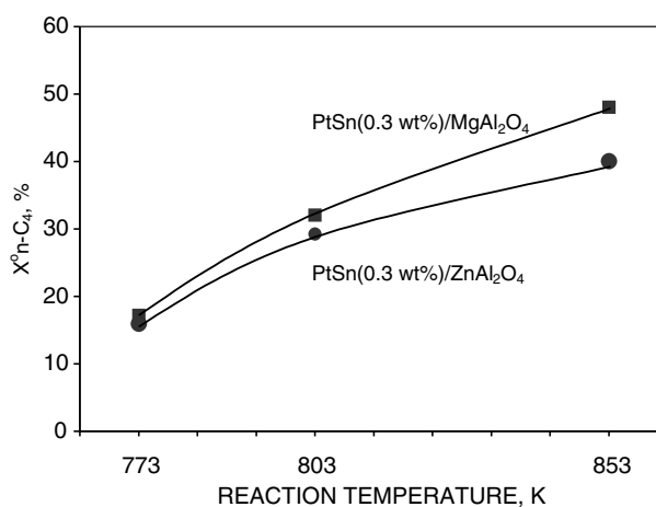
Figure 3. Effect of the reaction temperature on the initial n -butane conversion ( X^0_{n-C_4} ) for PtSn(0.3 wt%)/MgAl 2 O 4 and PtSn(0.3 wt%)/ZnAl 2 O 4 catalysts.
