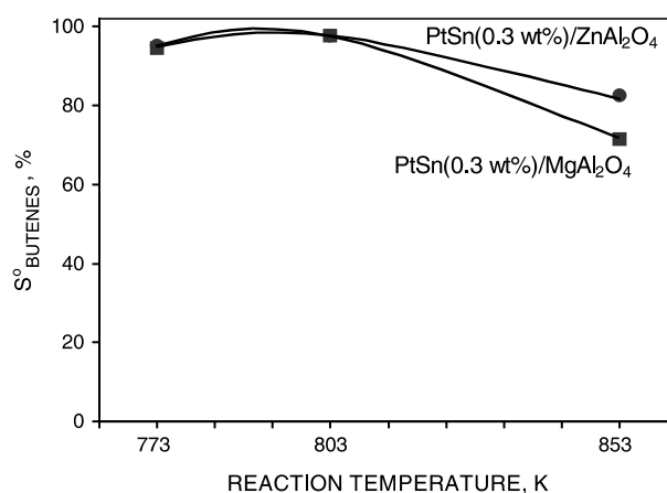
Figure 4. Effect of the reaction temperature on the initial selectivity to all butenes ( S^0_{BUTENES} ) for PtSn(0.3 wt%)/MgAl 2 O 4 and PtSn(0.3 wt%)/ZnAl 2 O 4 catalysts.
