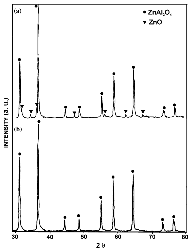
Figure 1. XRD spectra of non-purified ZnAl 2 O 4 (a) and purified ZnAl 2 O 4 (b).
