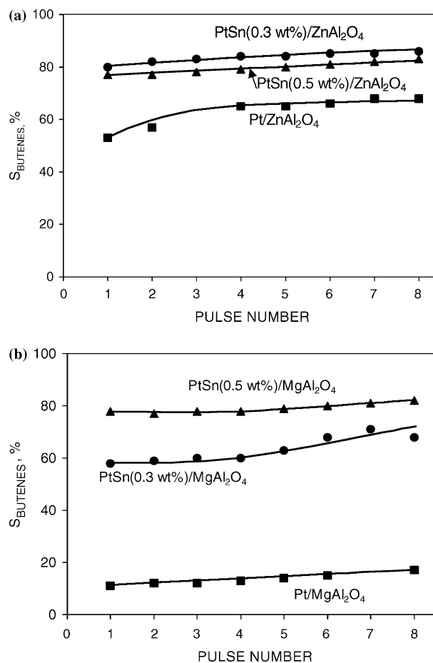
Figure 11. Selectivity to all butenes ( S BUTENES , %) as a function of the pulse number for catalysts supported on ZnAl 2 O 4 (a) and for catalysts supported on MgAl 2 O 4 (b). Pulse experiments at 803 K.
